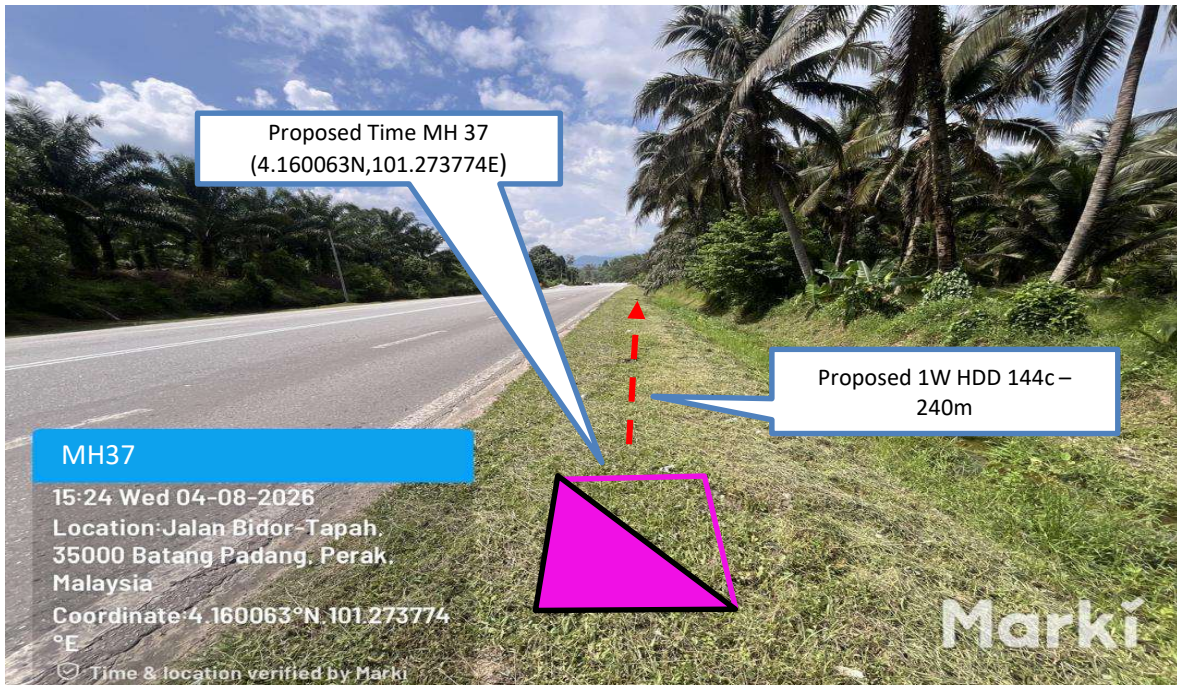
Prop 1W HDD 144C from Proposed Time MH37 n to Proposed Time MH38- 240 m
