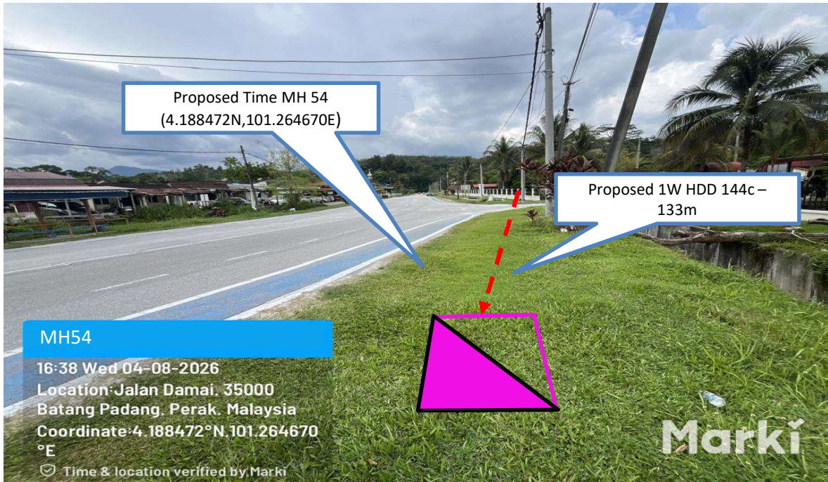
Prop 1W HDD 144C from Proposed Time MH53 n to Proposed Time MH54– 133 m
