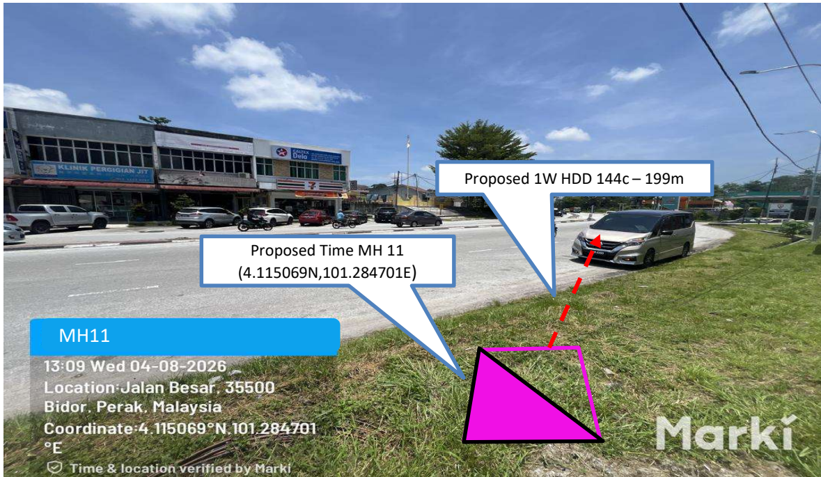
Prop 1W HDD 144C from Proposed Time MH11 n to Proposed Time MH12 – 199 m
