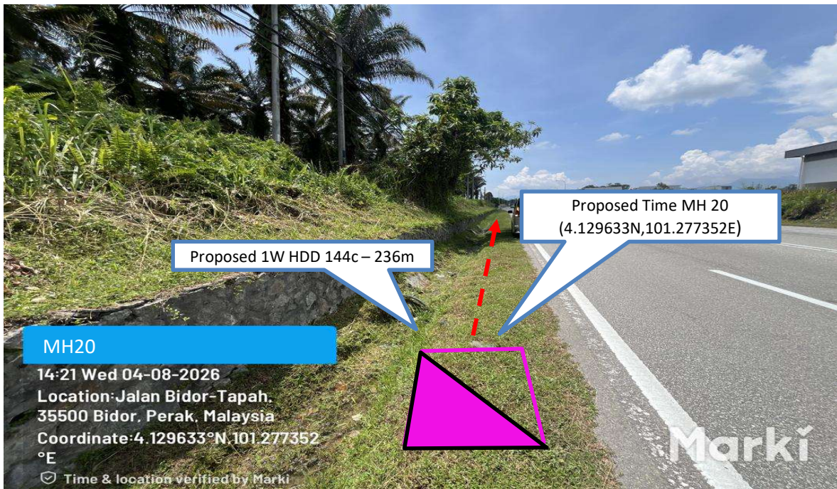
Prop 1W HDD 144C from Proposed Time MH20 n to Proposed Time MH21 - 236m
