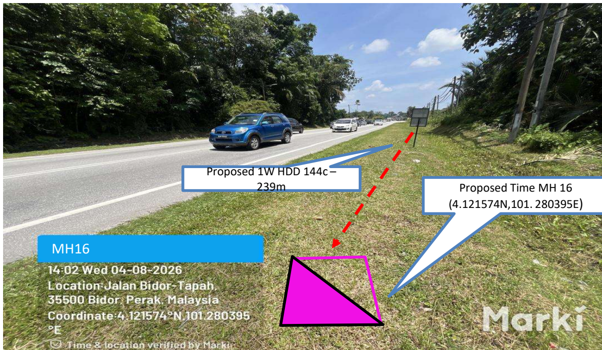
Prop 1W HDD 144C from Proposed Time MH15 n to Proposed Time MH16 - 239 m
