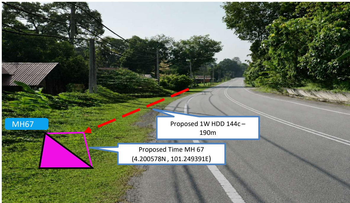
Prop 1W HDD 144C from Proposed Time MH66 n to Proposed Time MH67-190M
