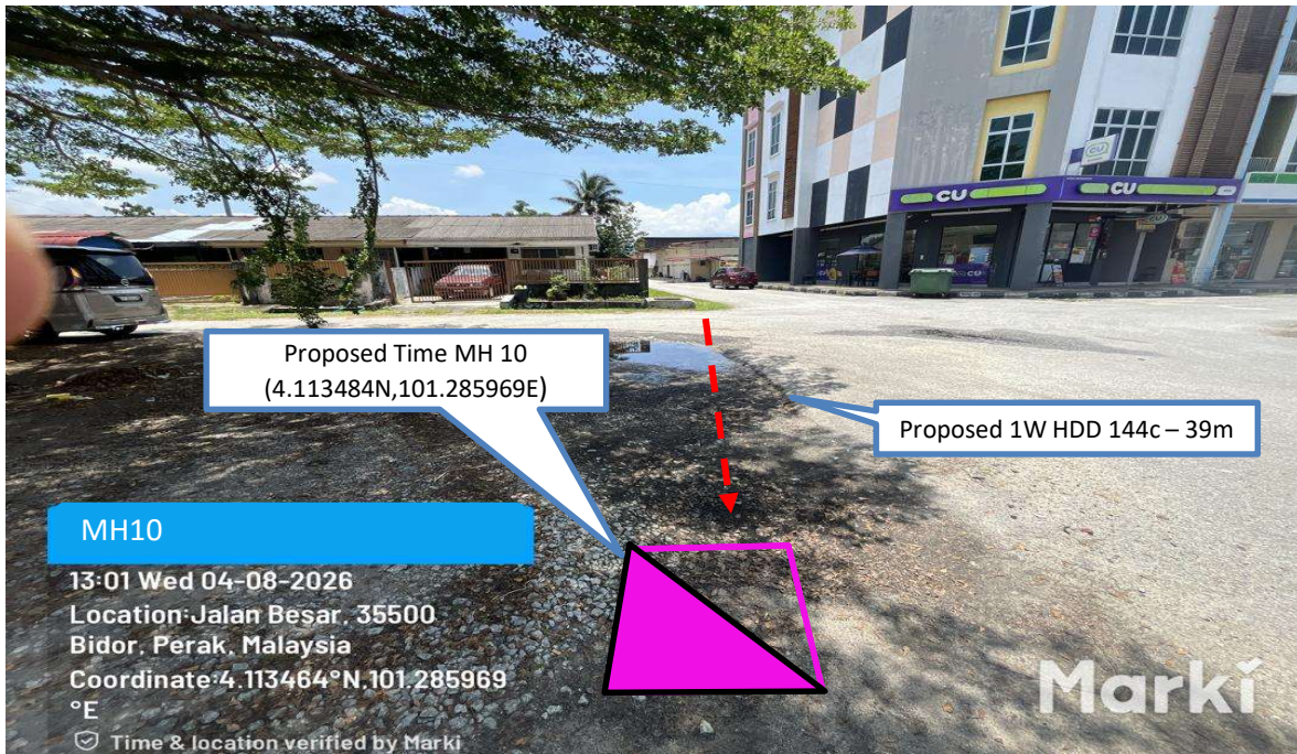
Prop 1W HDD 144C from Proposed Time MH09 n to Proposed Time MH10 – 39 m
