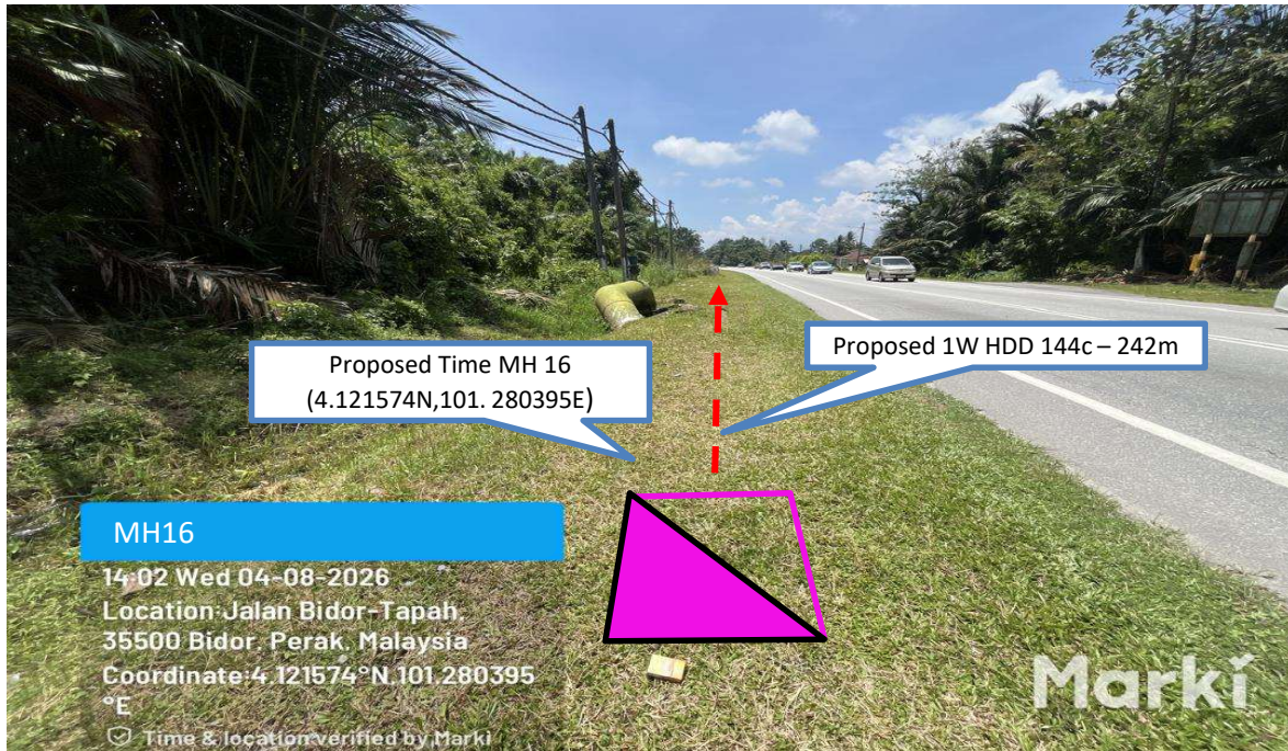
Prop 1W HDD 144C from Proposed Time MH16 n to Proposed Time MH17 - 242 m
