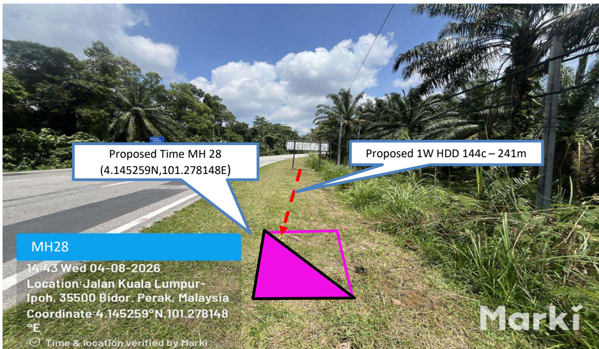
Prop 1W HDD 144C from Proposed Time MH27 n to Proposed Time MH28 – 241m
