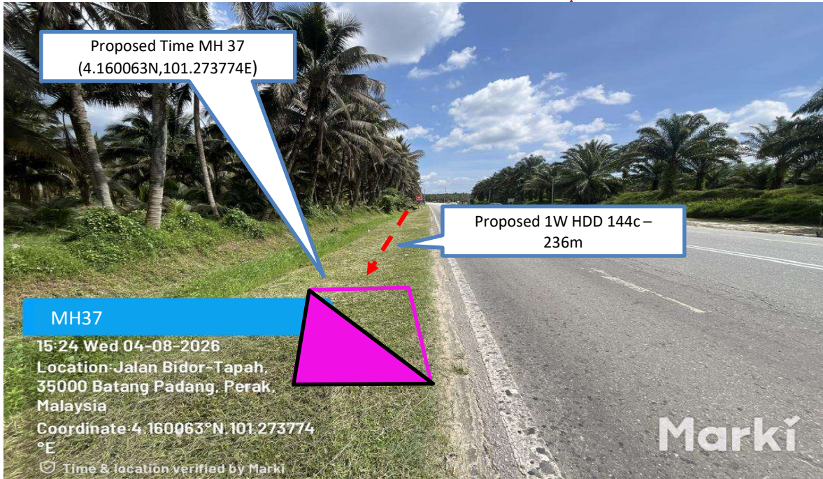
Prop 1W HDD 144C from Proposed Time MH36 n to Proposed Time MH37- 236 m
