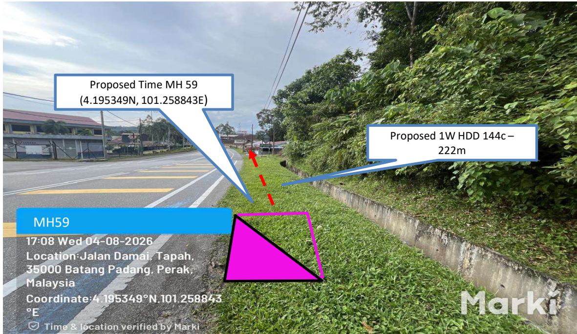
Prop 1W HDD 144C from Proposed Time MH59 n to Proposed Time MH60– 222 m
