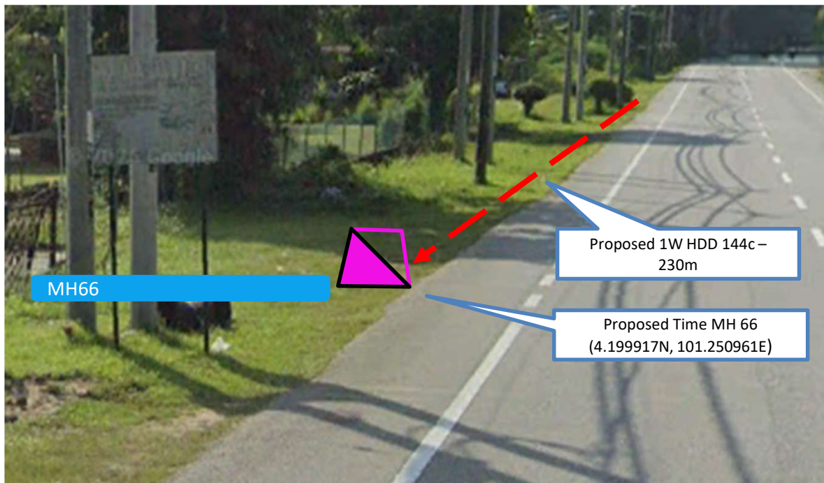
Prop 1W HDD 144C from Proposed Time MH65 n to Proposed Time MH66-230M
