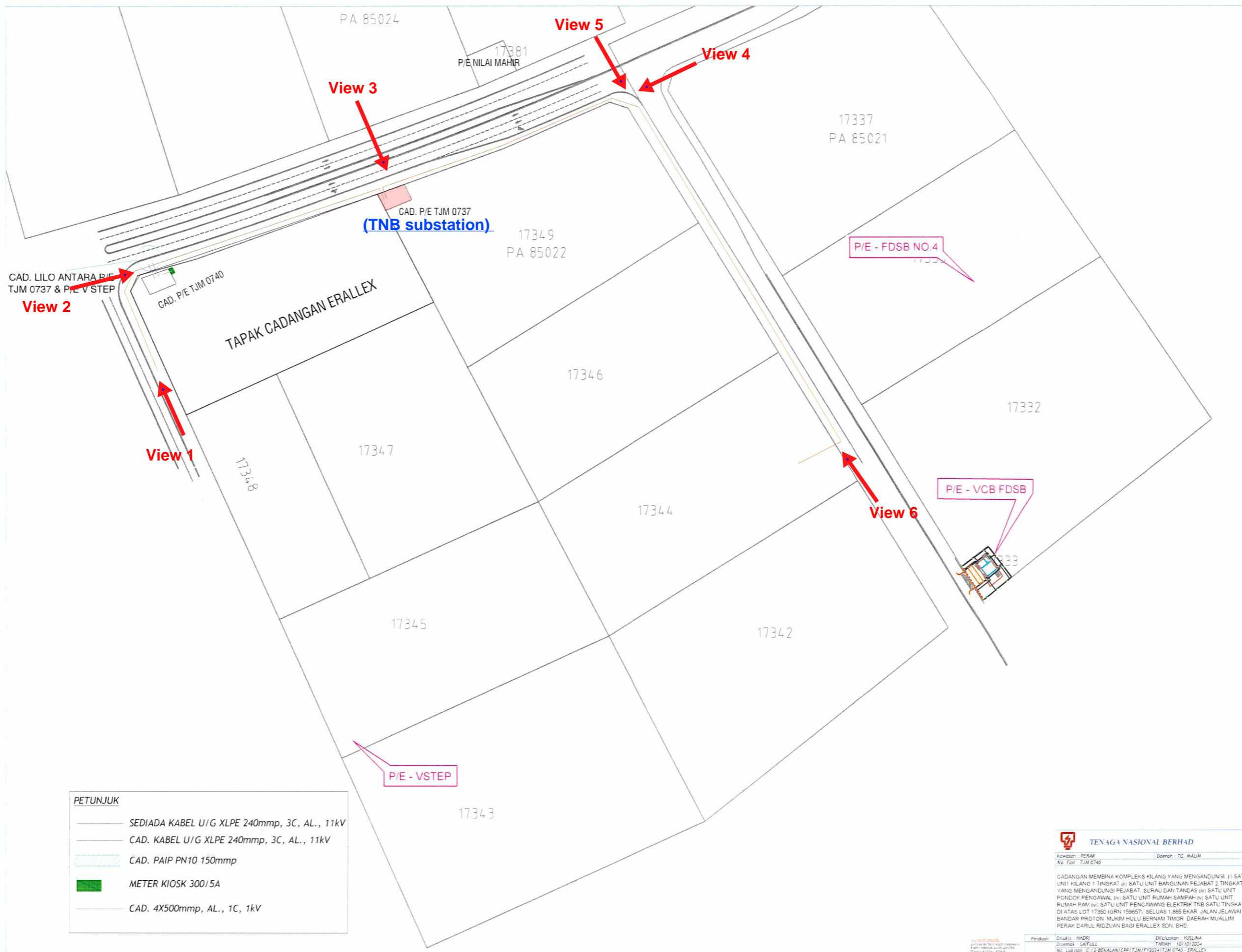
GAMBAR LOKASI TAPAK LOT 17349 - TNB SUBSTATION TRILLION SPEED
