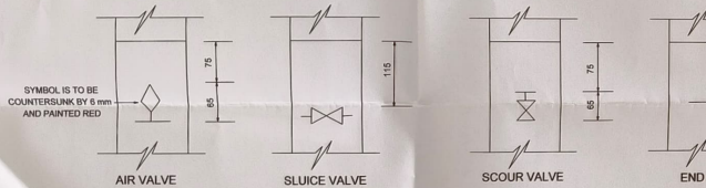
DETAIL AT "B" STANDARD FOR PIPE MARKER
