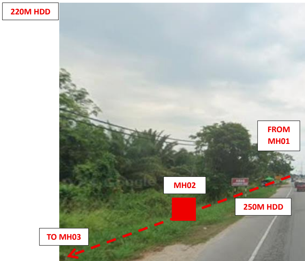
PICTURE 4 : FROM PROPOSE MH01 TO PROPOSE MH02
