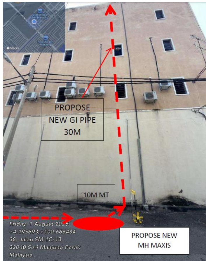
PICTURE 4 : PROPOSE MAXIS MH AND MICROTRENCH 10M
