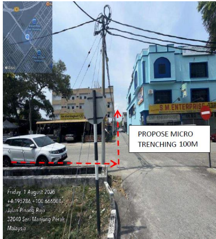
PICTURE 3 : PROPOSE MICROTRENCH 100M TO PROP MAXIS MH
