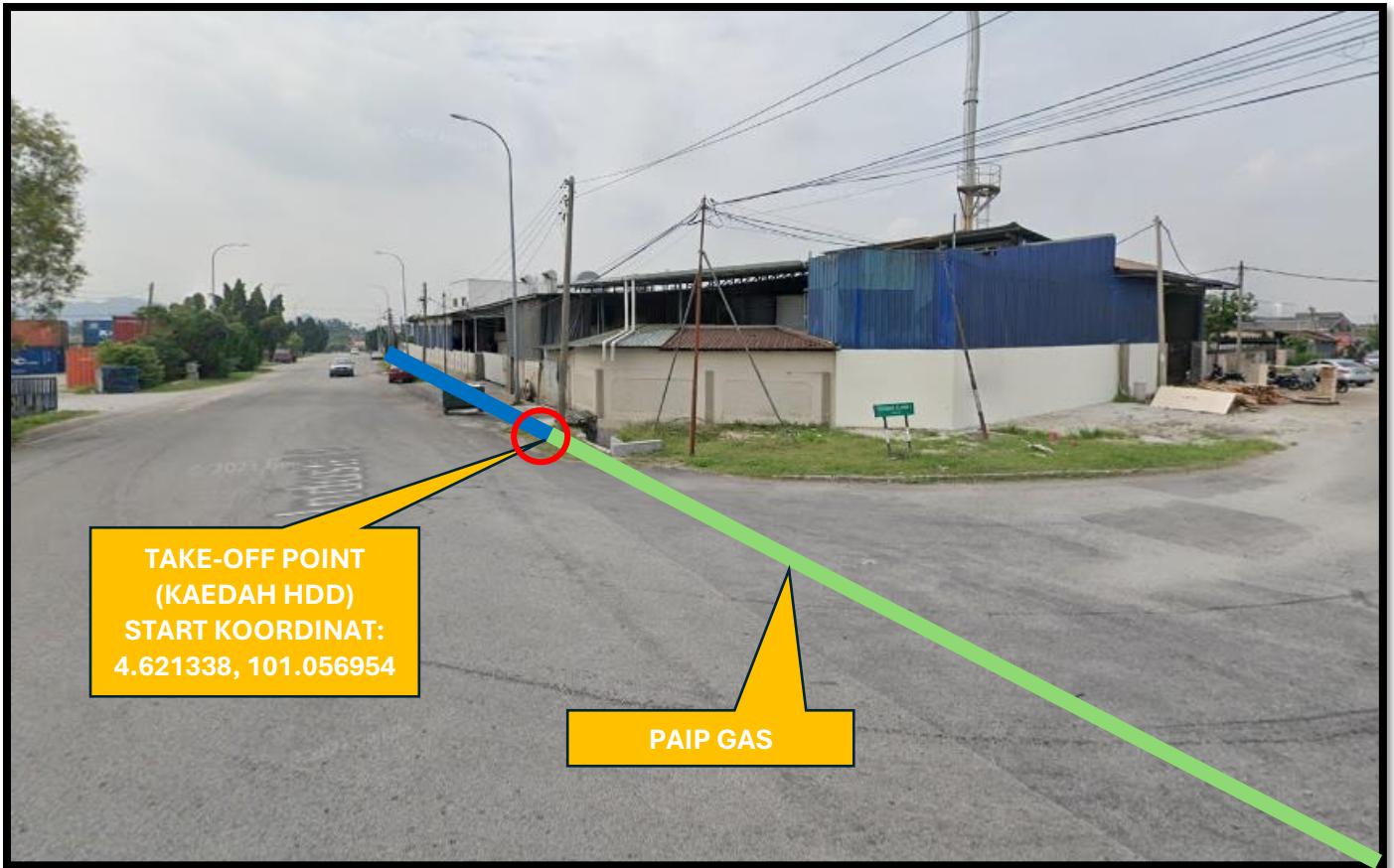
FIGURE 1.2: JALAN INDUSTRI 1
