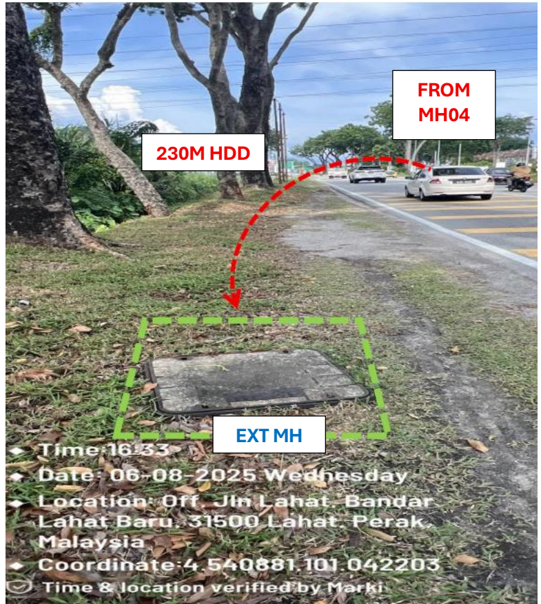
PICTURE 7 : EXISTING MAXIS MANHOLE
