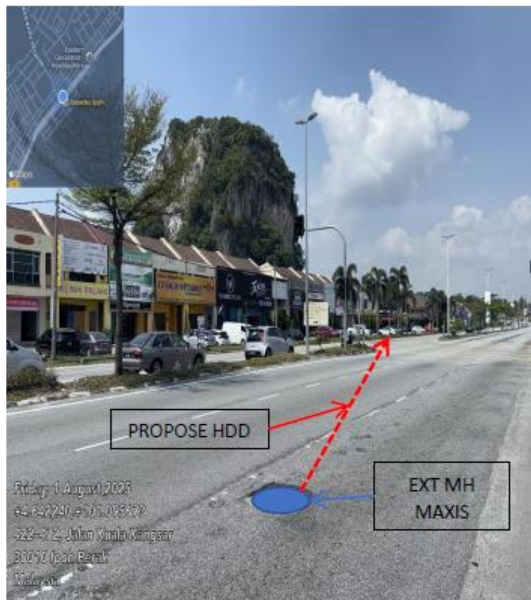
PICTURE 2 : PROPOSE 160M HDD WORK TO PROP MH01
