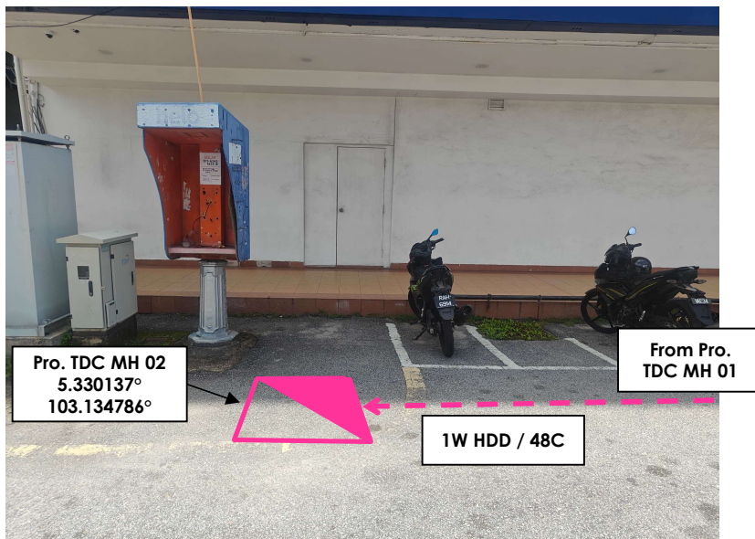
Propose route along Jalan Ungkusan – HDD Method
