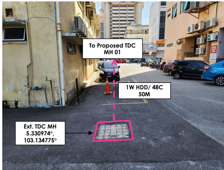
Propose route along Jalan Banggol – HDD Method
