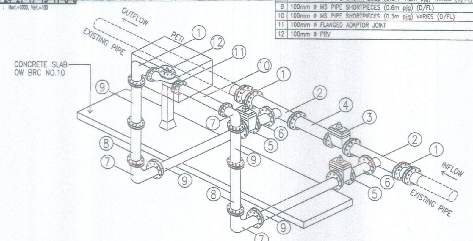
PRESSURE REDUCING VALVE (PRV) DETAIL
