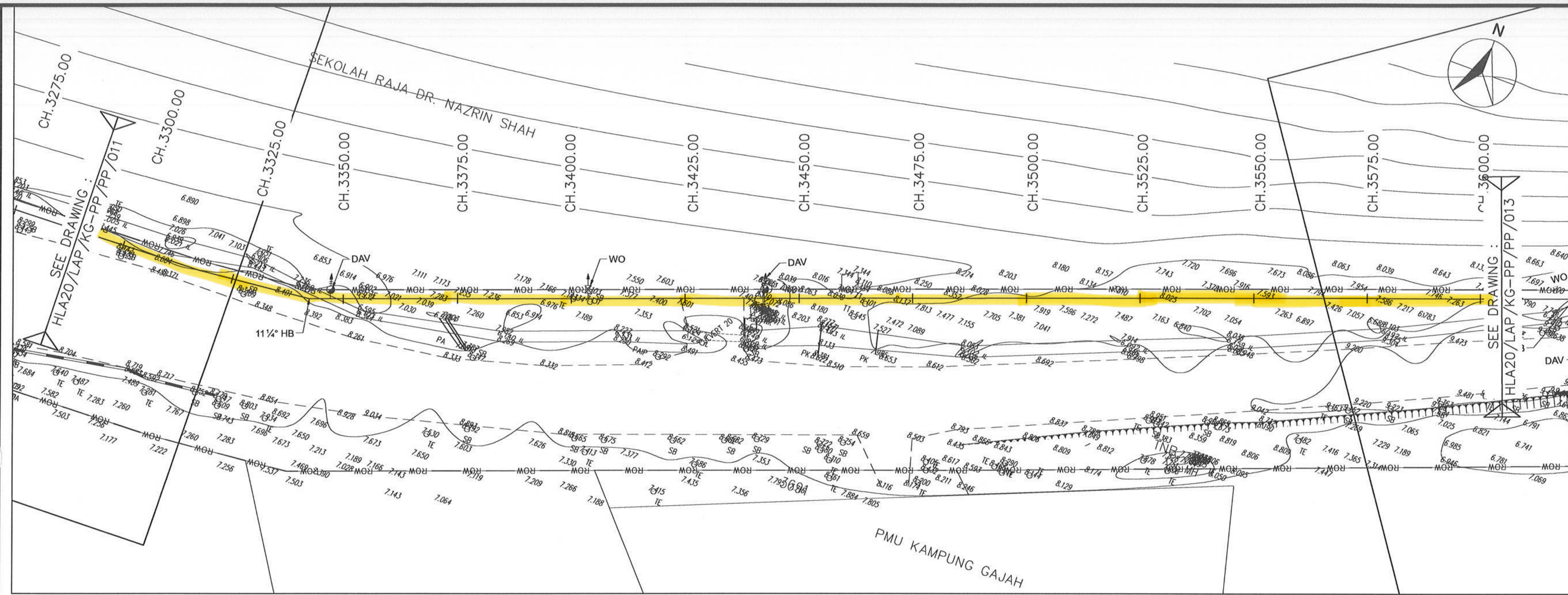
PLAN SCALE 1:500
