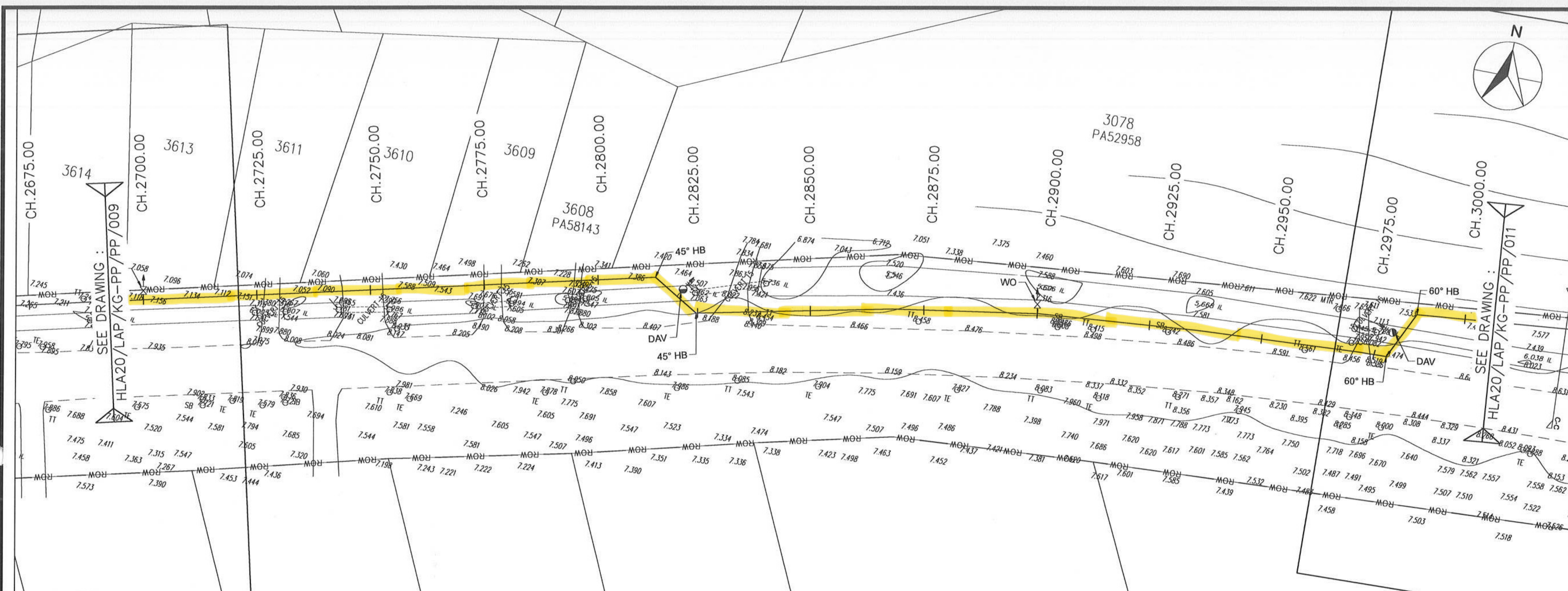
PLAN SCALE 1:500
